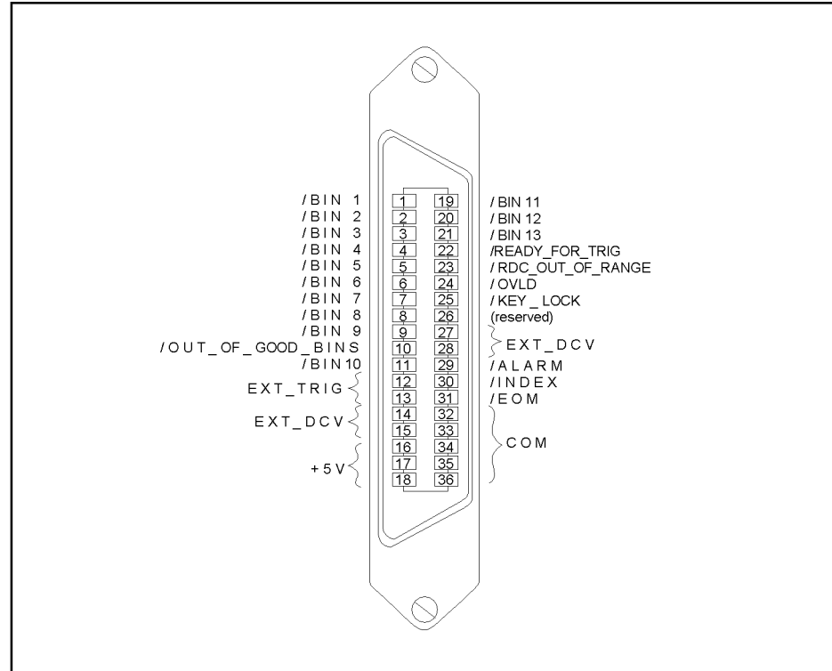
Description of the handler Interface Input/Output Signals
