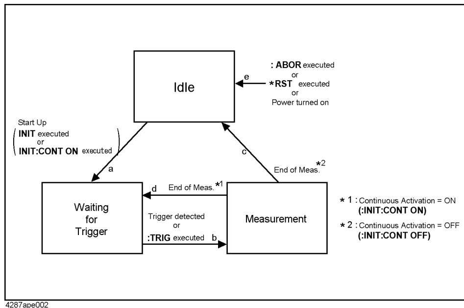
Trigger system
