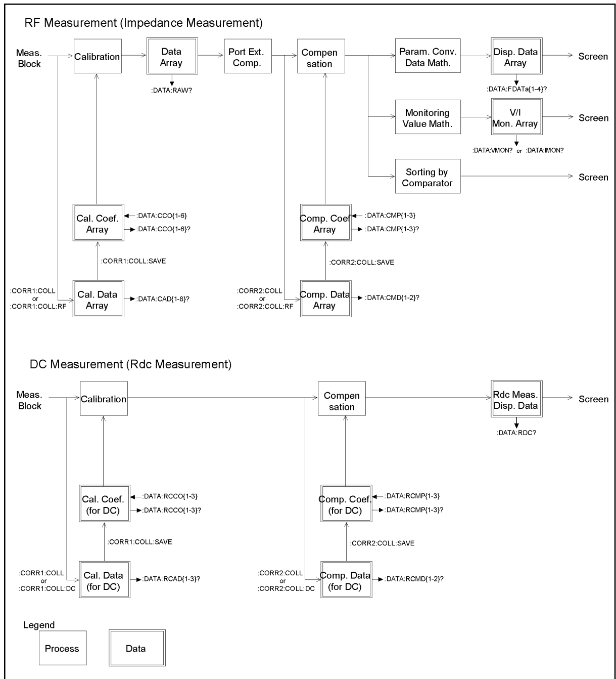
Figure 6-5 4287A's data processing flow
